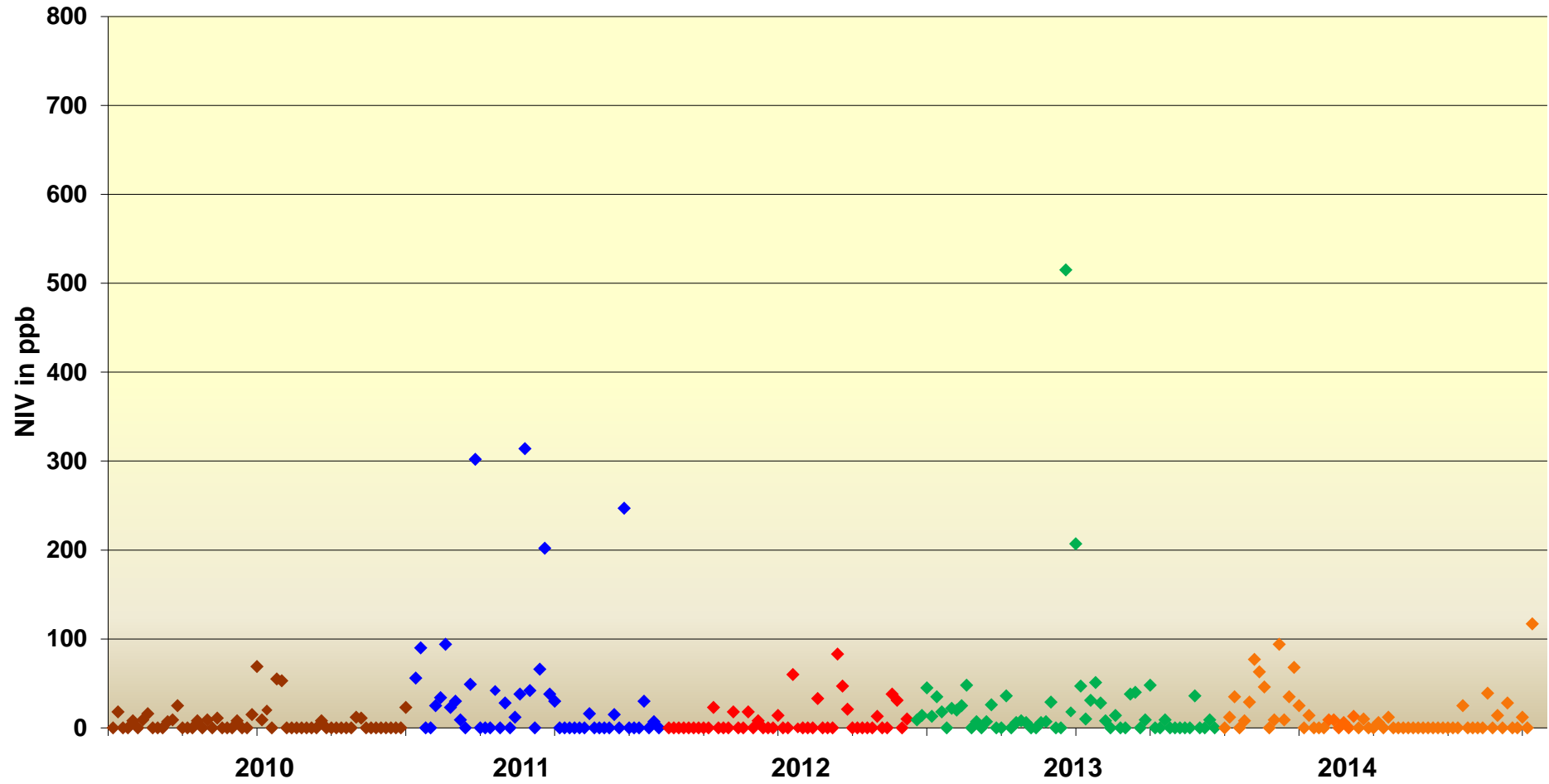
NIV \mu\text{g}/\text{kg} in UK Barley from crop years 2010 to 2014
