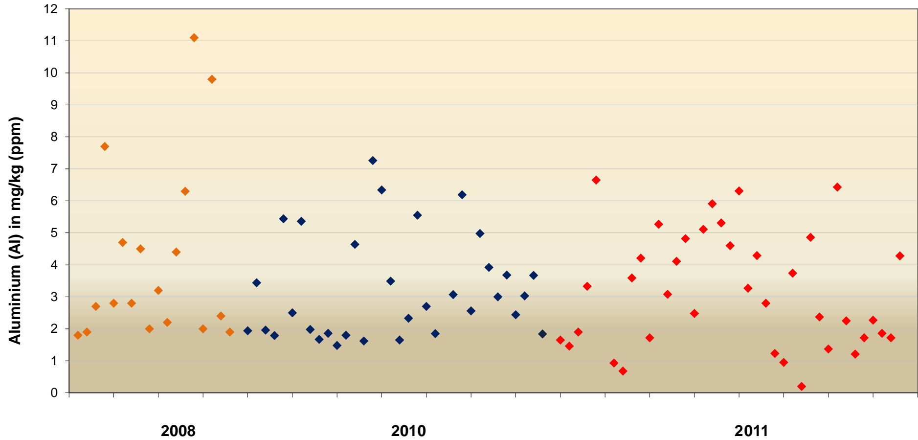
Aluminium (Al) tests carried out on UK Malting Barley in crop years 2008 to 2011
