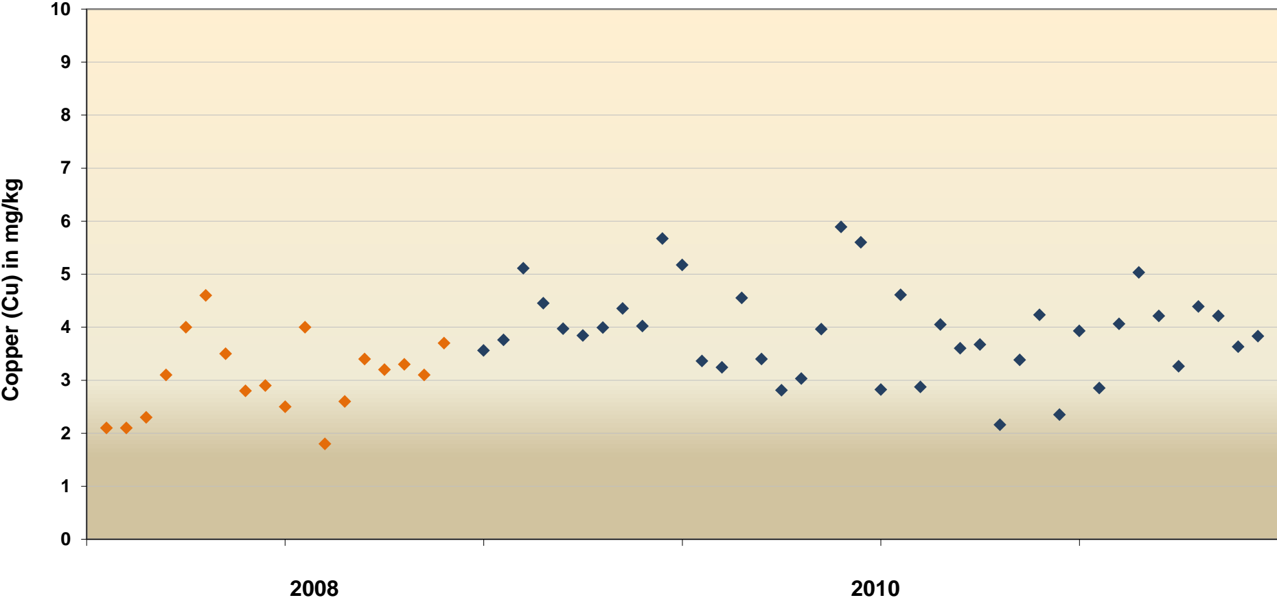
Copper (Cu) tests carried out on UK Malting Barley in crop Years 2008 to 2010
