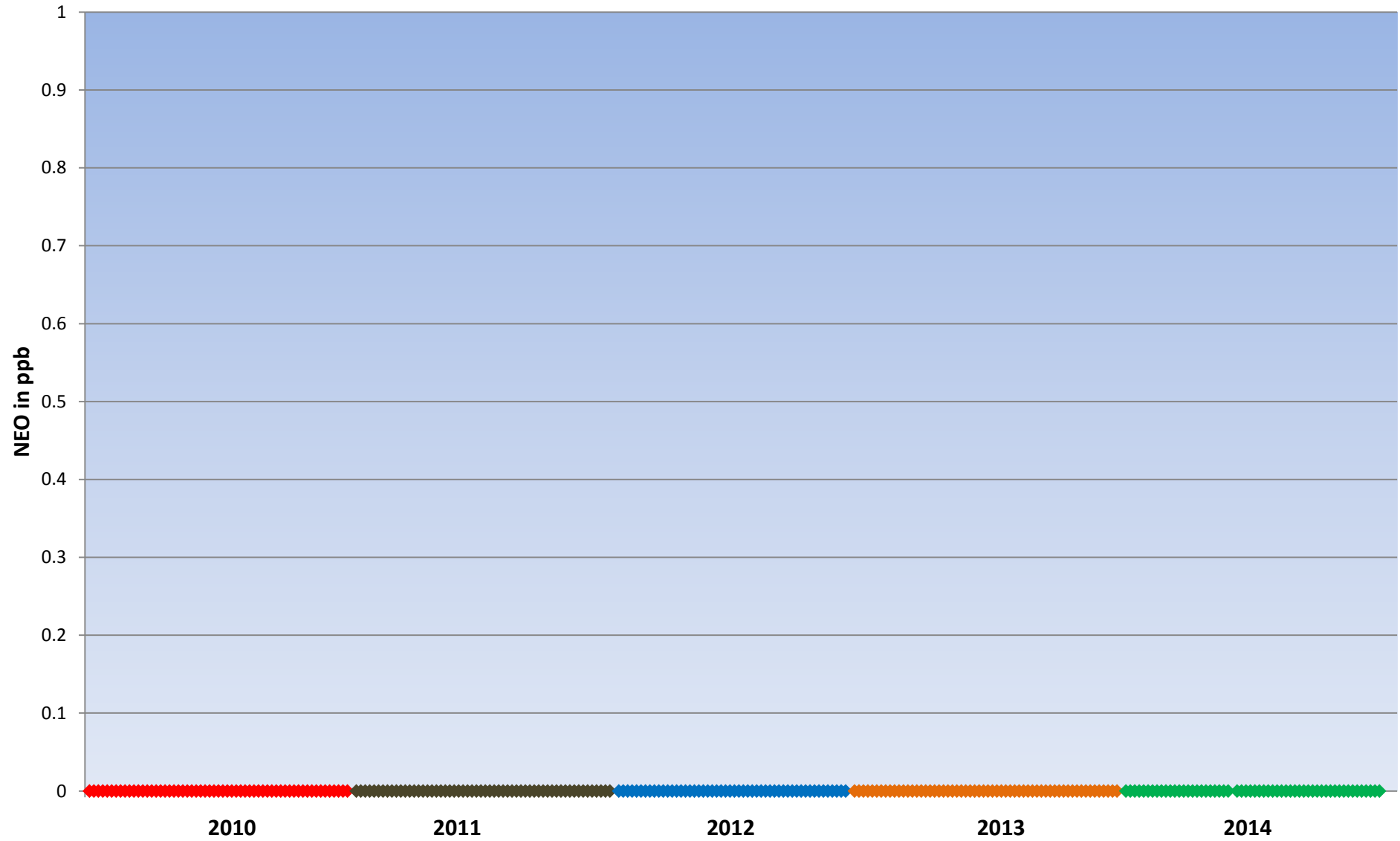
Neosolaniol (NEO) \mu\text{g}/\text{kg} in UK Barley from 2010 to 2014 crop years
