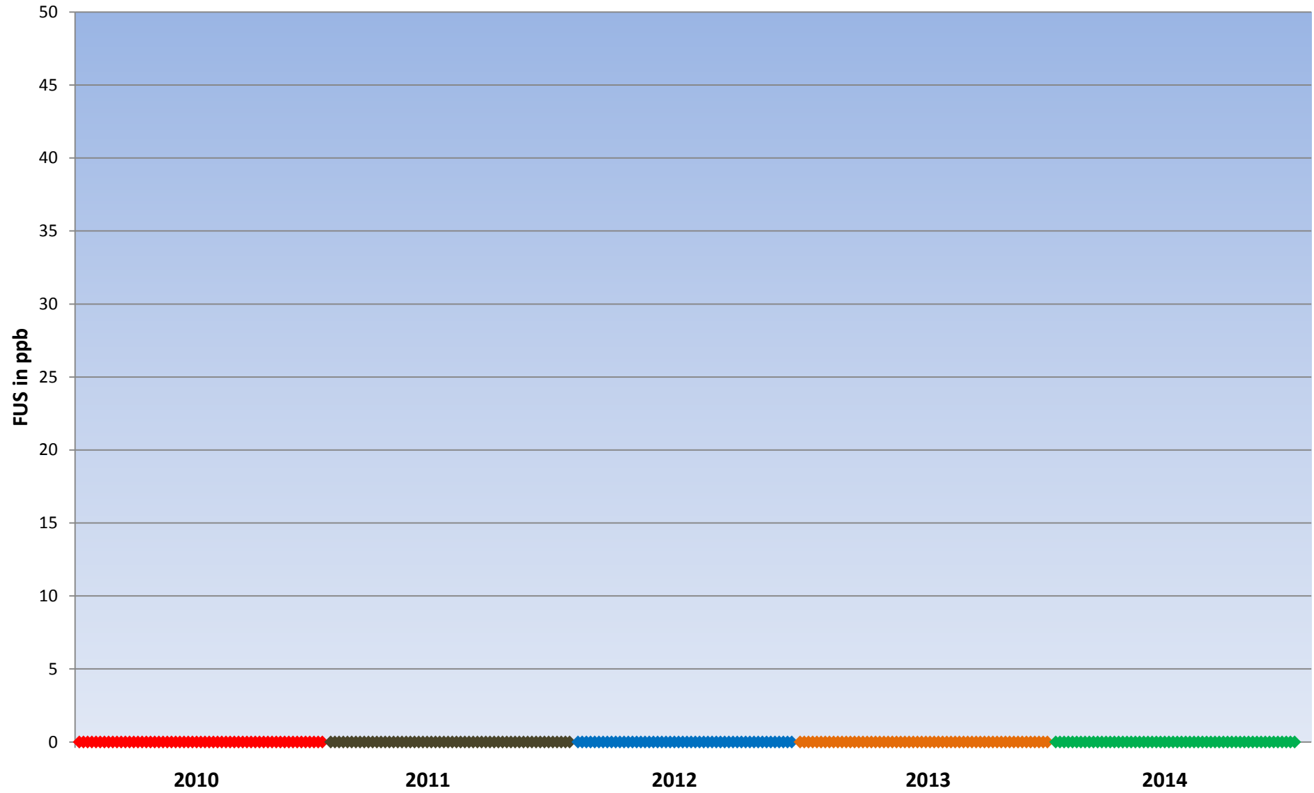
Fusarenone-X (FUS) \mu\text{g}/\text{kg} in UK Barley from 2010 to 2014 crop years
