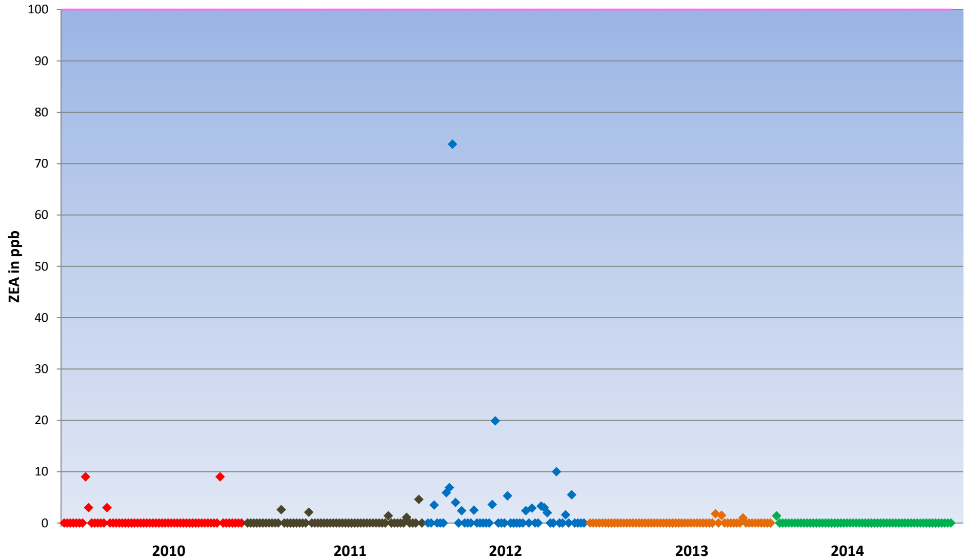
Zearalenone \mu\text{g}/\text{kg} in UK Barley from 2010 to 2014 crop years. (EU MRL was set at 100 ppb ( \mu\text{g}/\text{kg} ) in unprocessed cereals in 2007)
