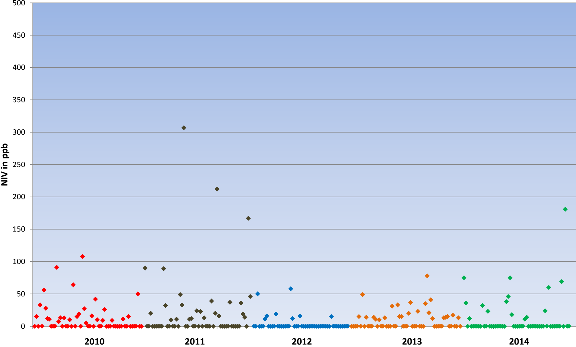
NIV \mu\text{g}/\text{kg} in UK Barley from crop years 2010 to 2014
