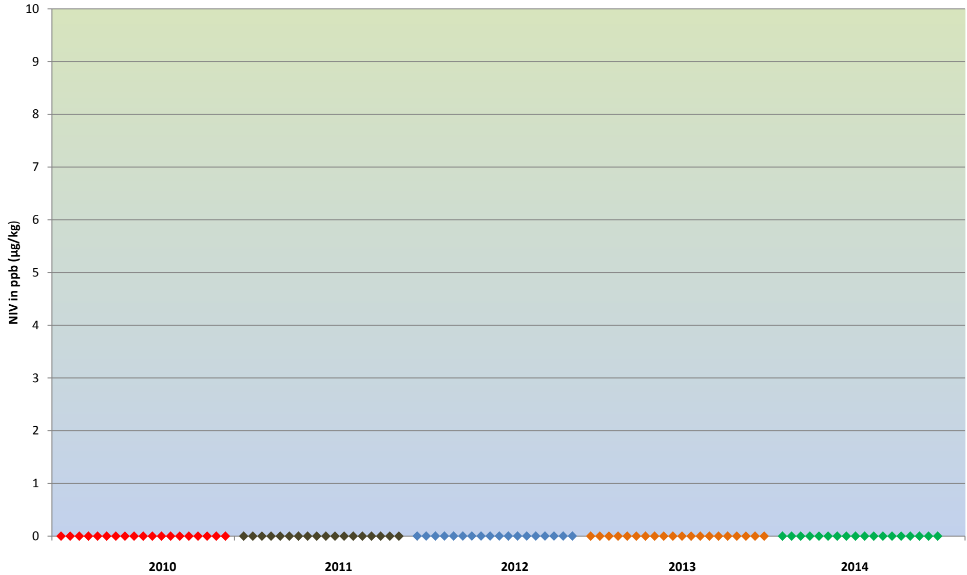
NIV in Malt made from barley in crop years 2010 to 2014
