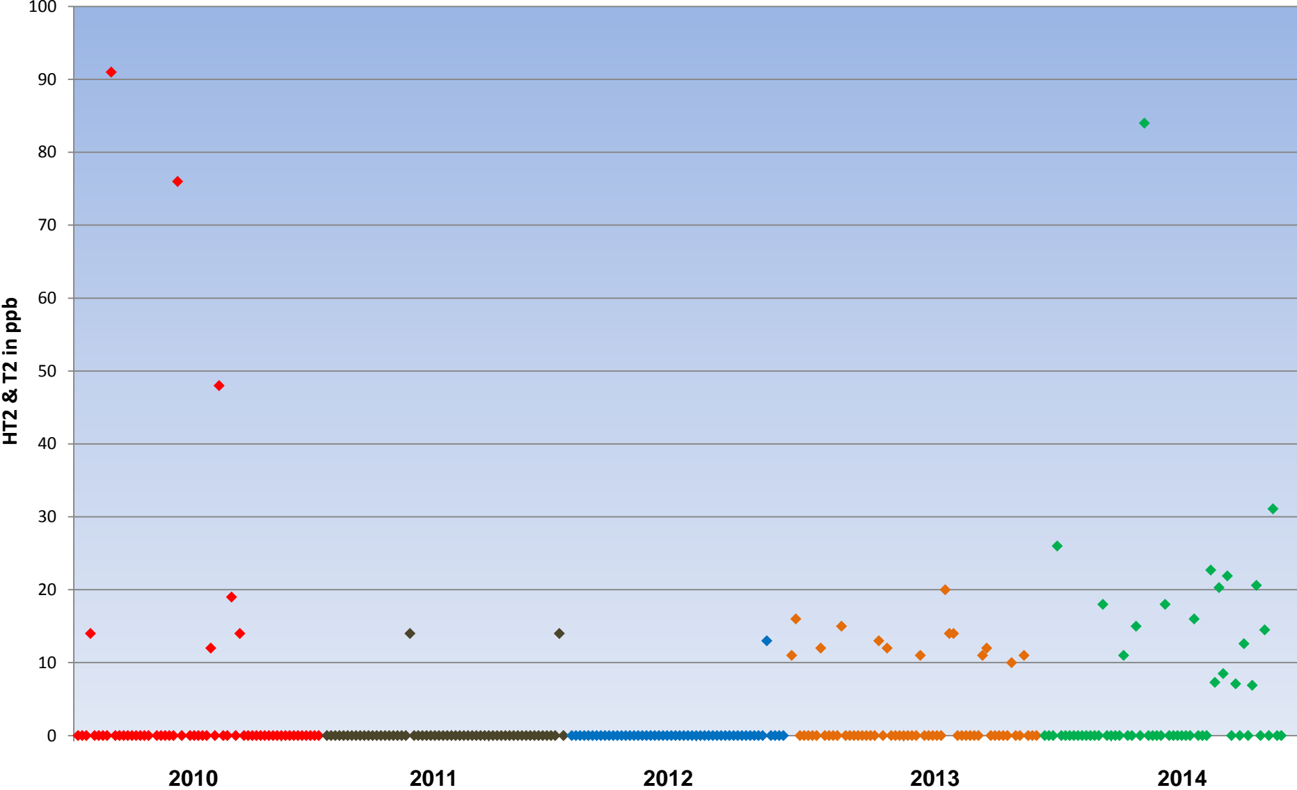
HT2 & T2 \mu\text{g}/\text{kg} in UK Barley from crop years 2010 to 2014
