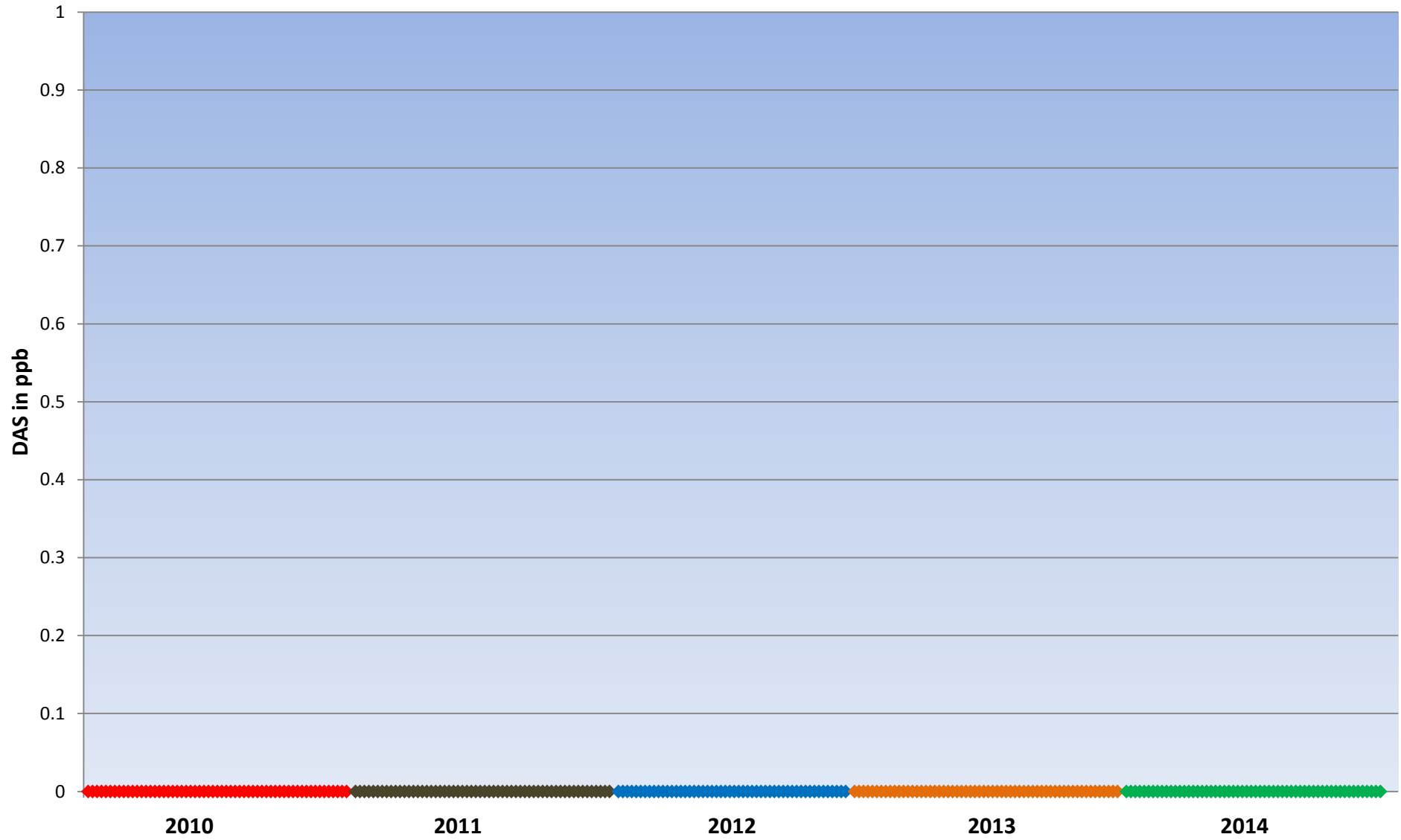
Diacetoxyscirpenol (DAS) \mu\text{g}/\text{kg} in UK Barley from 2010 to 2014 crop years
